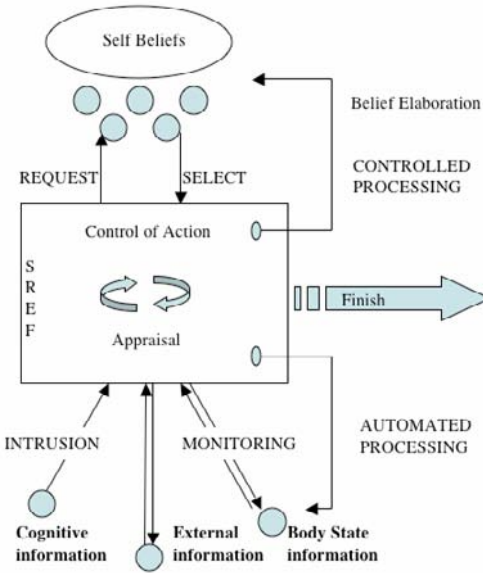
Fig. 3. SREF model
